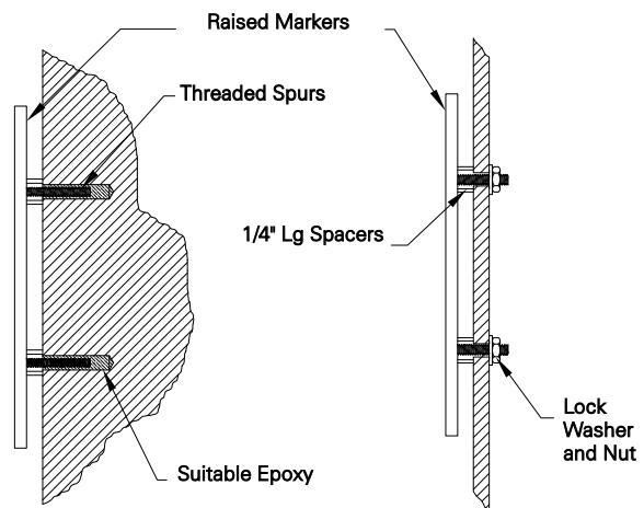
CONVENTIONAL WALL
